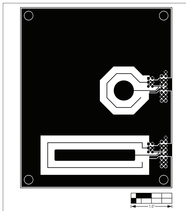
Figure 14. MAX1441TP EV Kit PCB Layout—Component Side
